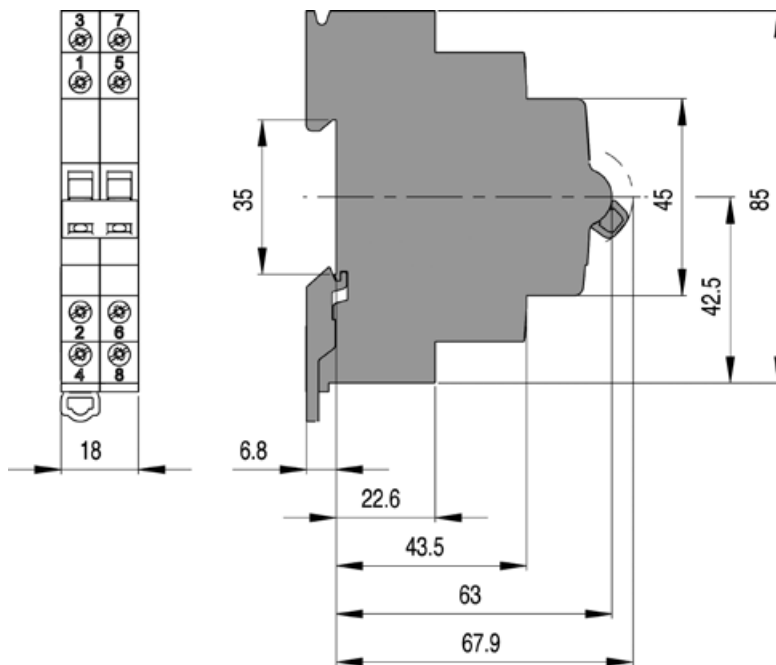
Switch, 3+4-pole
