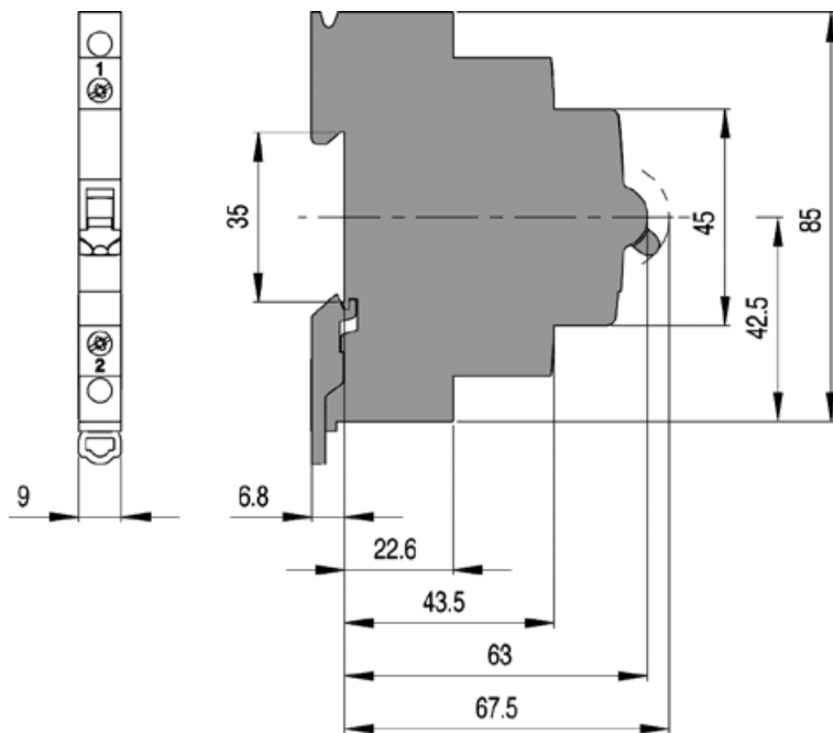
Switch, 1+2-pole
