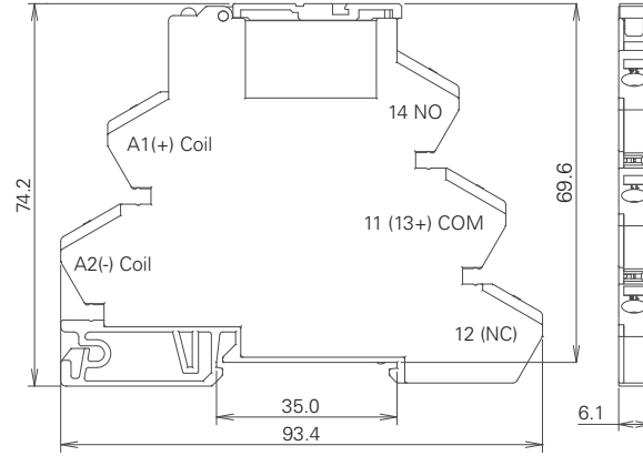
RV8H-S Spring Clamp Terminal (mm)
