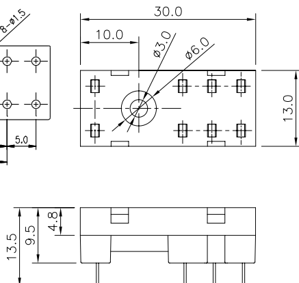
SQ2V-63
