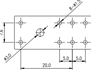
SQ2V-63 PCB Pin Layout
